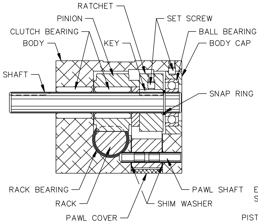
SIDE VIEW
