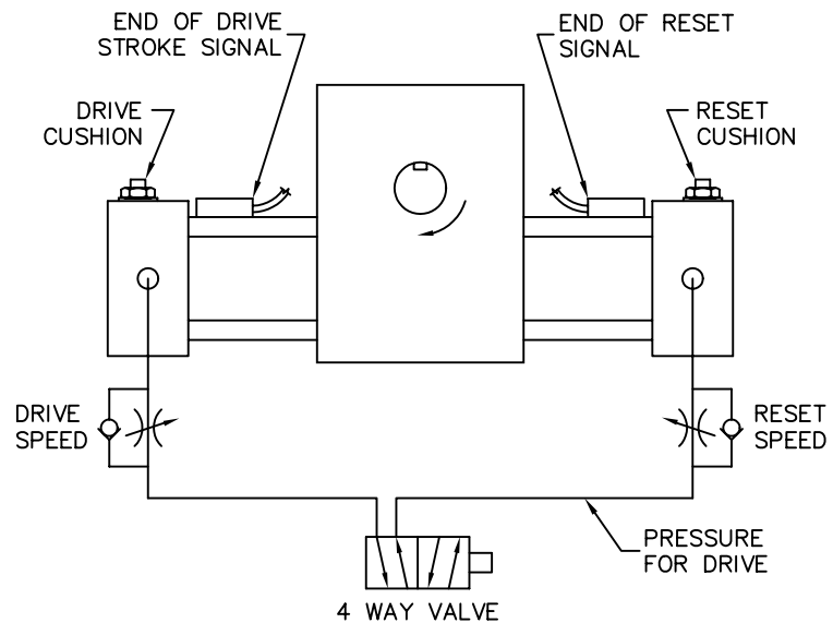
CLOCKWISE ACTUATOR
