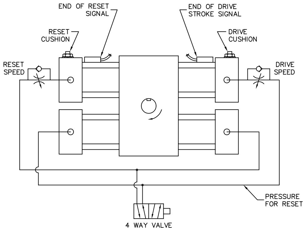
CLOCKWISE ACTUATOR
